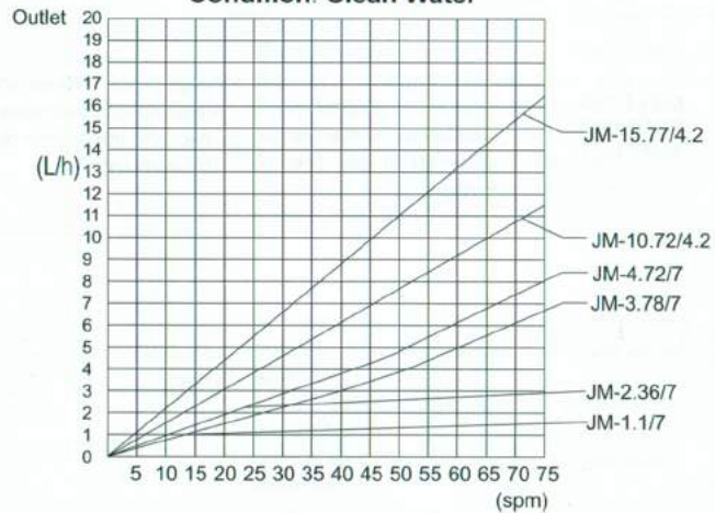
Performance Curve Drawing Condition: Clean Water
