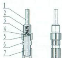
INJECTION VALVE
